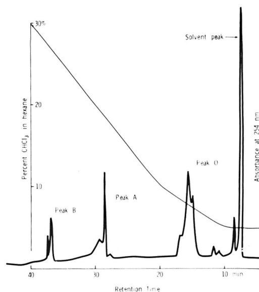
FIG. 2. Adsorption chromatography of fatty acids with more than 1000 molecular weight. Elution was performed with a linear gradient of CHCl 3 from 0–30% in n-hexane. The flow rate was fixed at 1 ml/min.
