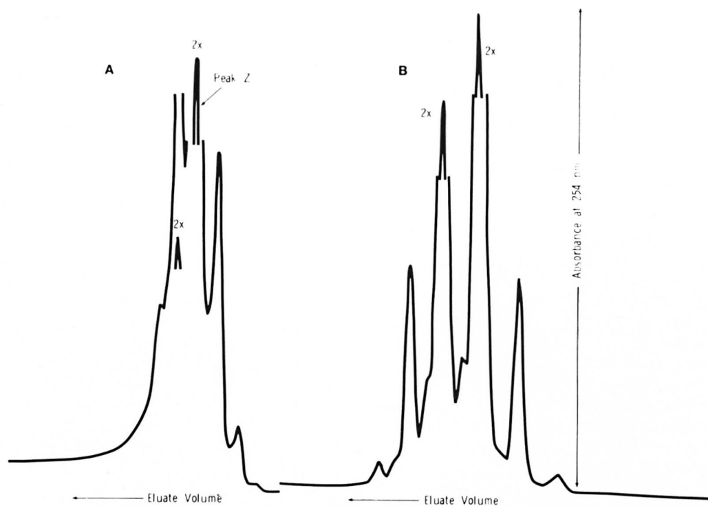
FIG. 10. Reverse-phased chromatography of mycolic acids of M. lepraemurium grown in vitro . The chromatographic conditions in Figs. 10A and 10B were the same as in Figs. 3A and 3B, respectively.
