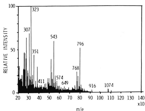
FIG. 13. Mass-spectrum of one of the main mycolic acids of mycobacteria collected from the liver of an armadillo with naturally acquired leprosy-like disease. An Hitachi M-80 mass-spectrometer was used.
