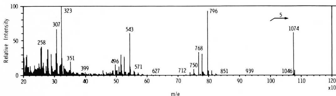
FIG. 4. Mass-spectrum of one of the main mycolic acids from the footpad of a nude mouse with leprosy. An Hitachi M-70 mass-spectrometer was used.
