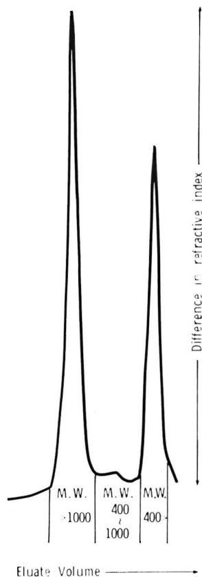
FIG. 6. Gel-permeation chromatography of the total fatty acids in mycobacteria collected from the liver of an armadillo with experimental leprosy. A refractometer was used as the detector. Other conditions were the same as Fig. 1.
