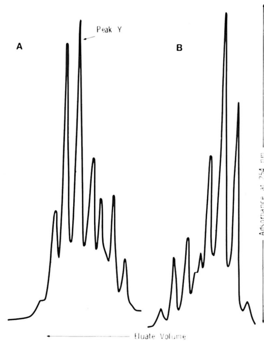
FIG. 7. Reverse-phased chromatography of mycolic acids of mycobacteria collected from the liver of an armadillo with experimental leprosy. The chromatographic conditions in Figs. 7A and 7B were the same as in Figs. 3A and 3B respectively.
