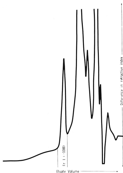
FIG. 1. Gel-permeation chromatography (GPC) of the total fatty acids in the footpad of a nude mouse with leprosy. The flow rate of the eluting solvent (THF) was fixed at 2 ml/min.
