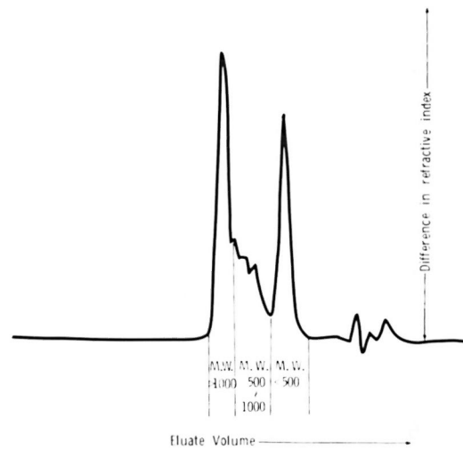
FIG. 9. Gel-permeation chromatography of the total fatty acids in M. lepraemurium grown in vitro . The chromatographic conditions were the same as in Fig. 1.
