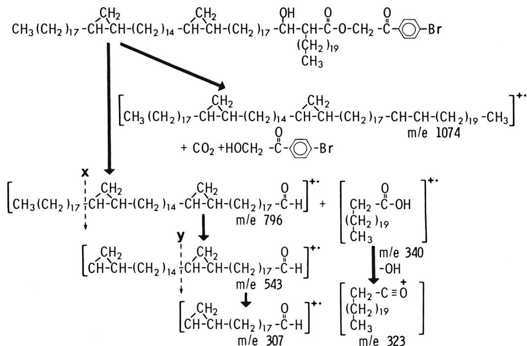
FIG. 5. Mass-fragmentation deduced from the spectrum of Fig. 4.
