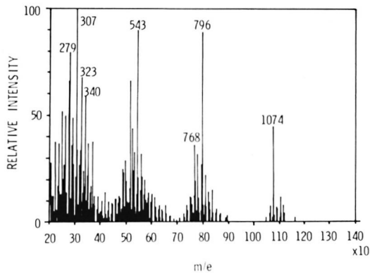
FIG. 8. Mass-spectrum of one of the main mycolic acids of mycobacteria collected from the liver of an armadillo with experimental leprosy. An Hitachi M-80 mass-spectrometer was used.
