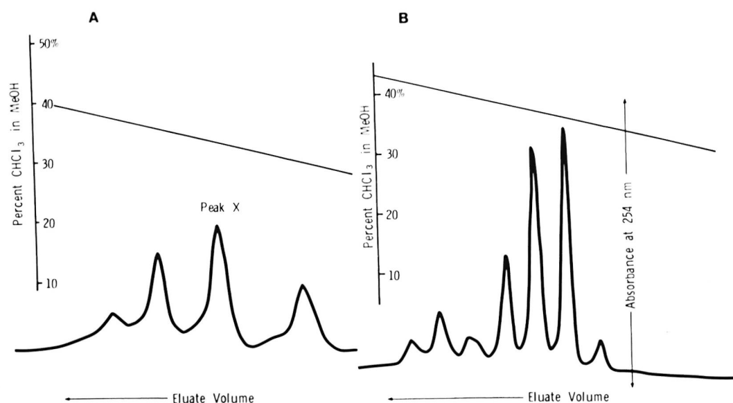
FIG. 3. Reverse-phased chromatography of eluates from the adsorption chromatography. A: eluate corresponding to peak A in Fig. 2. B: eluate corresponding to peak B in Fig. 2. Elution was performed with a linear gradient of \text{CHCl}_3 from 0–50% in methanol. The flow rate was fixed at 1 ml/min.
